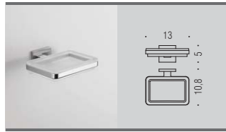
B3701 Porta sapone Soap dish holder
