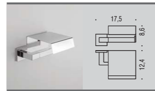
B3791 Porta rotolo coperto Paper holder with cover
